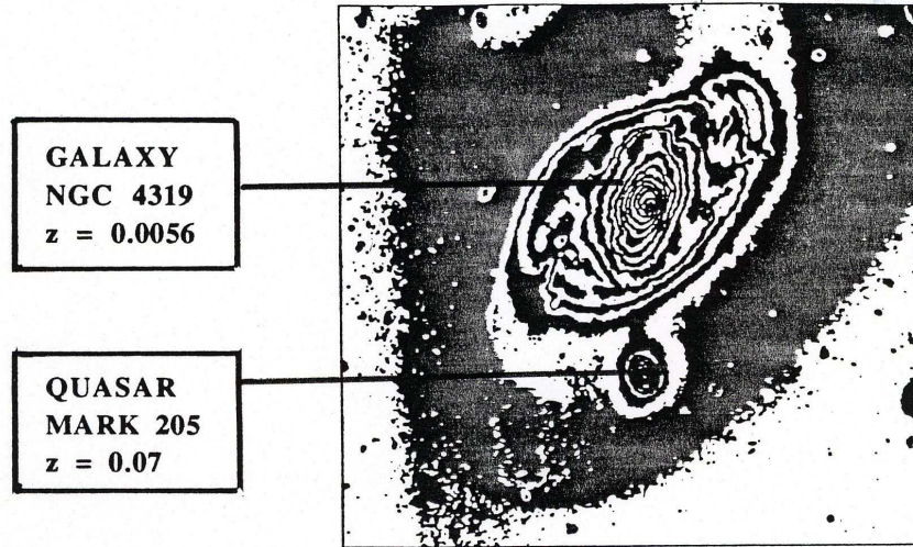
Figure 6.12. An example of clear evidence of astrophysical conditions beyond the capabilities of Einsteins special and general relativities or, equivalently, beyond the Minkowskian and Riemannian geometries: the experimentally verified (Ref. [67]) physical connection between the galaxy NGC 4319 and the quasar Mark 205, via the superposition of several gamma spectroscopic plates. By contrast, the quasar Mark 205 has a redshift with z = 0.07 , while the associated galaxy NCG 4316 has a redshift of only z = 0.0056 . The interpretation of this difference requires necessary departures from the Minkowskian and Riemannian geometries, because such a large difference would require that the quasar has at least 104 times the speed of the galaxy, under which conditions the quasar and its associated galaxy would have separated completely billions of years ago. Santilli's iso-Minkowskian geometry permits an exact, numerical, and invariant representation of the indicated large difference in cosmological redshifts, while restoring the abstract Minkowski and Poincaré axioms on isospaces over isofields.
