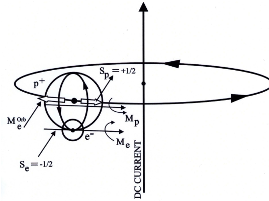
Figure 6.33. A schematic view of the pseudo-neutron expected from the collapse of the electron into the proton structure following the alignment of the preceding figure due to very strong, attractive, electric and magnetic Coulomb forces at 1F mutual distances due to opposing charges and magnetic polarities. Note that the coupling is in singlet, as necessary for any bond, and it is of axial character, namely, the spin of the proton and of the electron are initially aligned along a single symmetry axis. Following penetration inside the proton, the electron is expected to acquire conventional integer angular momenta, along the lines of Figure 6.23.
