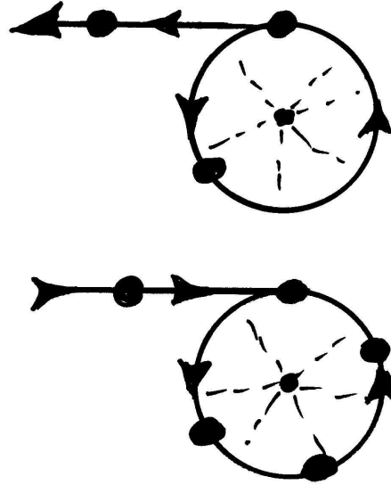
Figure 6.25. A schematic illustration of the inapplicability of Einstein's special relativity and its fundamental Poincaré symmetry for systems with constraints. The "sling shot" of this figure illustrates physical events impossible for special relativity and its Poincaré symmetry, but existing in the physical reality, such as the conversion of angular into linear momentum in the top view and the conjugate case of conversion of linear momentum into angular momentum in the lower view. When the physical reality of the neutron structure is admitted as being a constrained system, there is no need for the neutrino conjecture for both the neutron synthesis as well as for its decay. The understanding is that models without and with neutrinos do not necessarily exclude each other, the only scientific exclusion being that via unbiased experiments. The picture also illustrates the reason the author considers current "experimental results" in deep inelastic scattering as being "experimental beliefs." In fact, said results are claimed via the use of the conventional potential scattering theory under the notorious conditions of verifying Einsteinian doctrines and the Poincaré symmetry, thus (tacitly) excluding constrained conditions and exchanges of the type illustrated in this figure.
