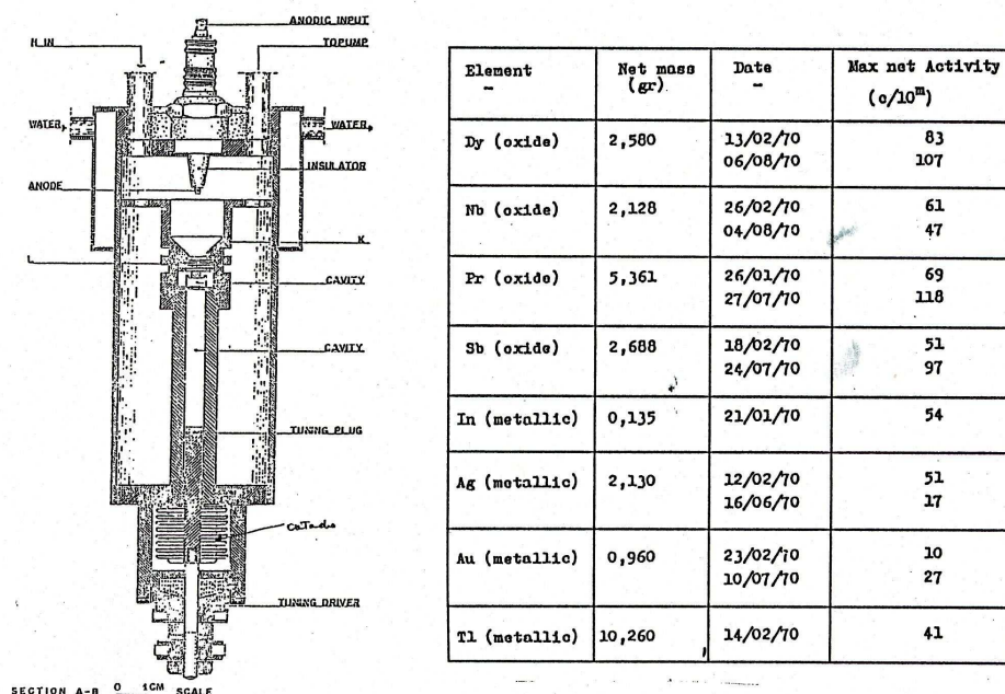
Figure 6.27. A view of the klystron used in tests [116,117] and one of the tables of results showing nuclear transmutations that can only occur via exposure to entities originating from the interior of the klystron, which entities have to be necessarily neutral and particle size (to pass through the metal wall of the klystron) and have strong interactions (to be absorbed by nuclei).
