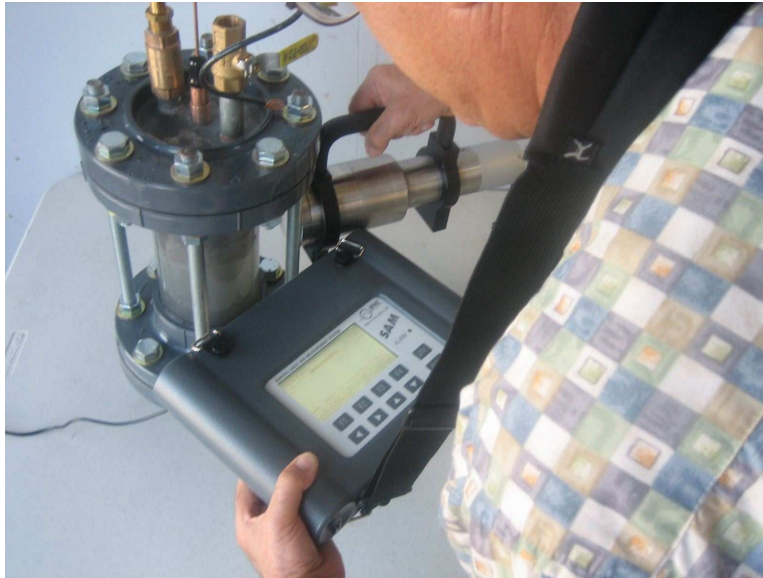
Figure 6.28. A picture of Klystron I and of detector SAM 935. Note the similarity with the klystron used in tests [116,117], but also the primary differences being given by the use of metal walls for tests [116,117], and transparent polycarbonate walls
